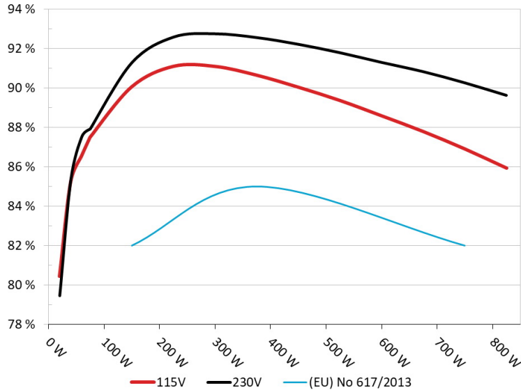
Efficiency: Corsair RM750x (Shift) Ambient: 37°C - 47°C (98.6°F - 116.6°F)
