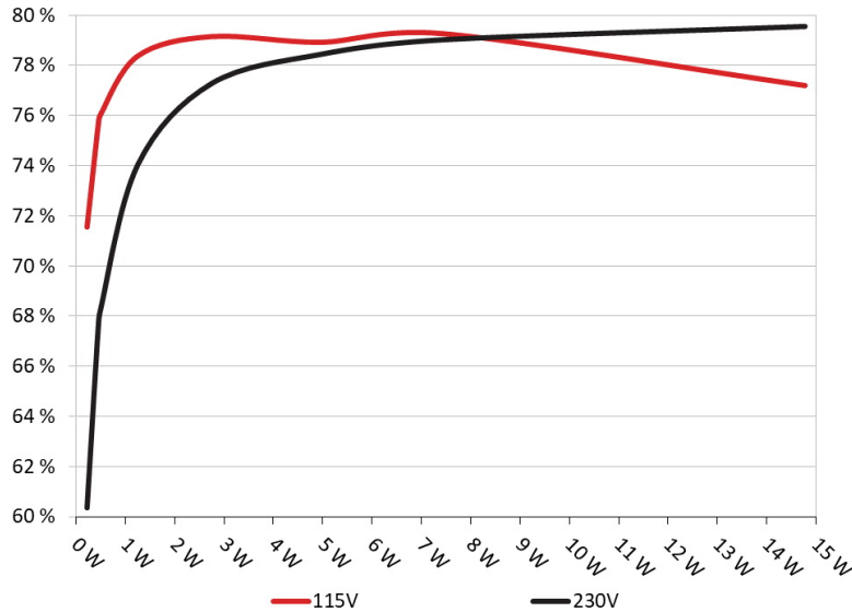
5VSB Efficiency: Corsair RM750x (Shift) Ambient: 34°C - 36°C (93.2°F - 96.8°F)
